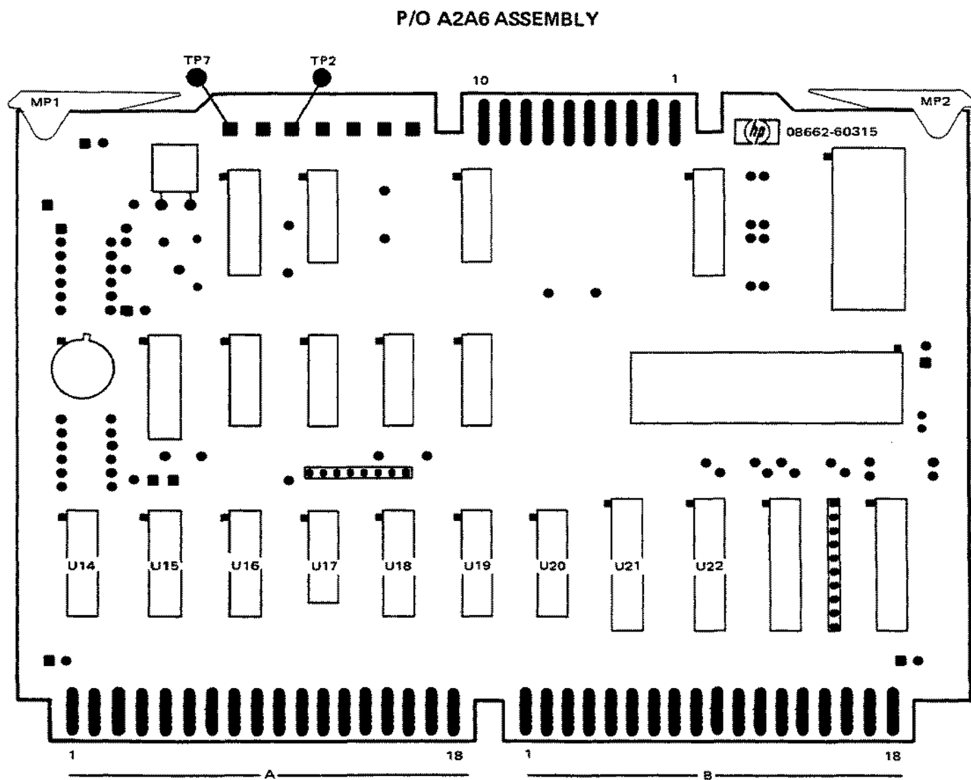
Figure 8-319. P/O A2A6 Microprocessor/Decoder Component Locations (P/O Change 10).
