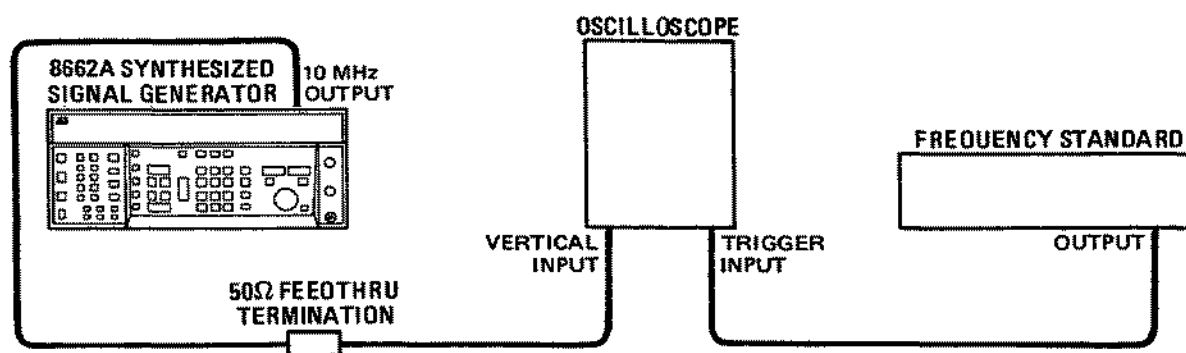
Figure 4-8. Internal Time Base Aging Rate Test Setup
