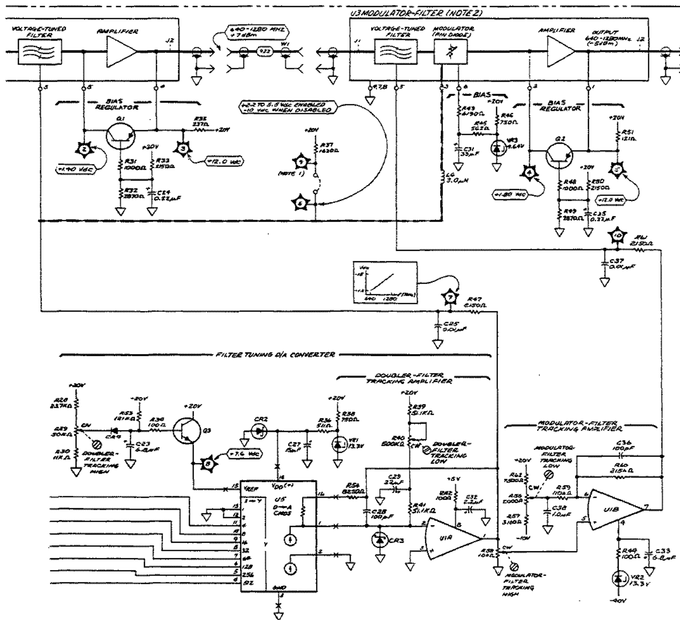
P/O Figure 8-512. A4A2 Output Section Douhler Schematic (P/O Change 4)
