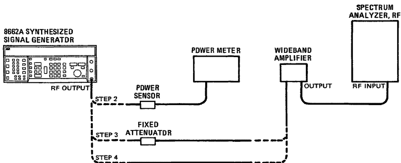
Figure 4-3. Level Accuracy Test Setup (Optional – Low Level)
