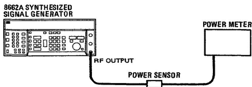
Figure 4-2. Level Accuracy and Flatness Test Setup
